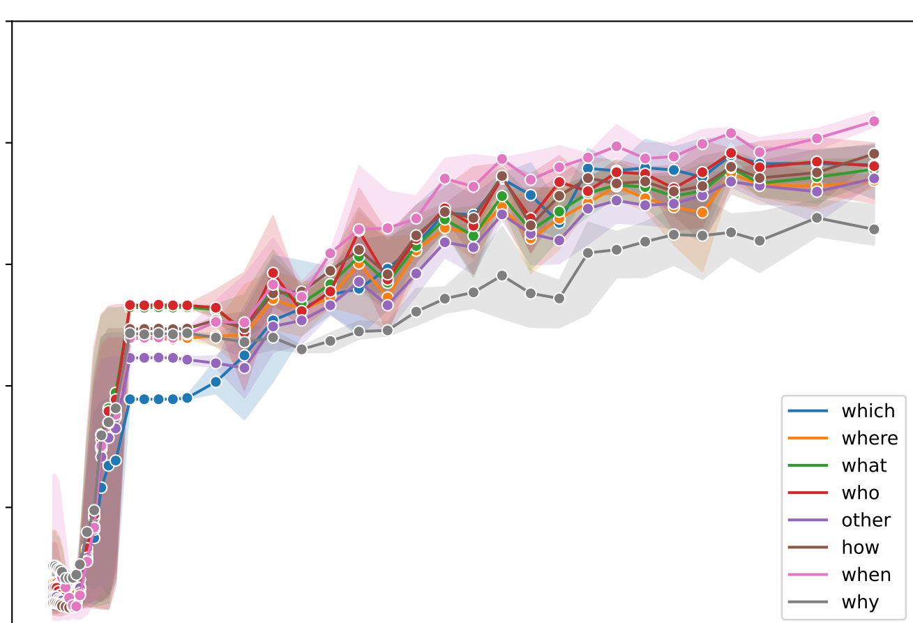
SQuAD 2.0
