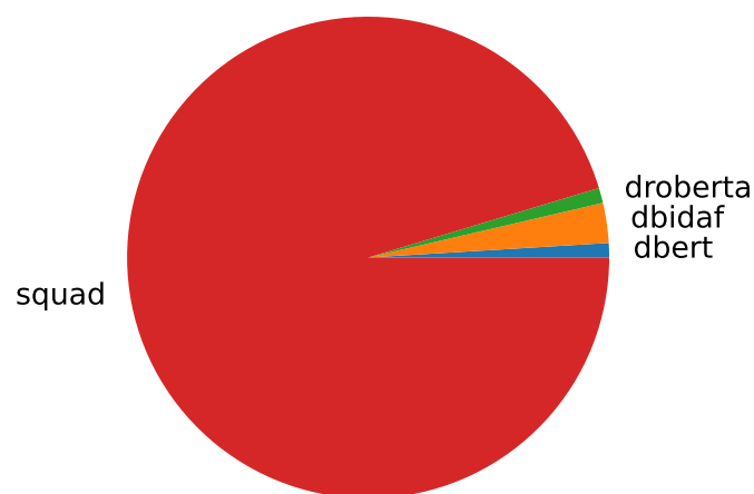
cluster 0 (n=1867)
