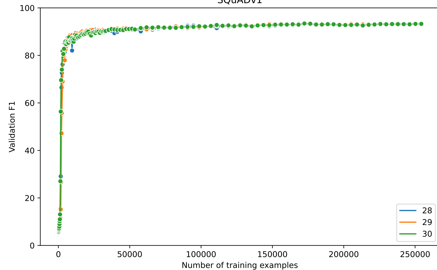
SQuADv1-AdQA
