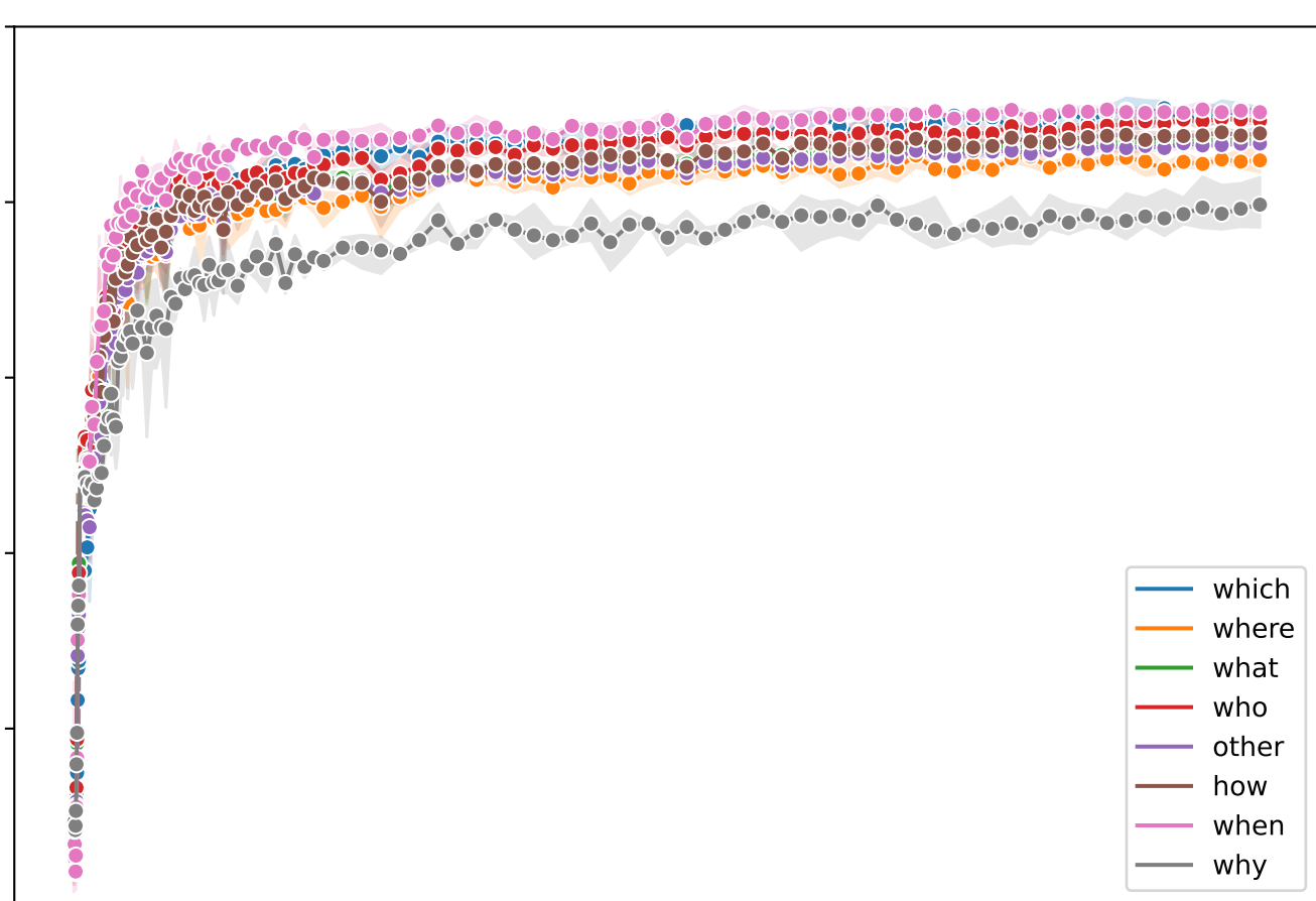
SQuAD 2.0
