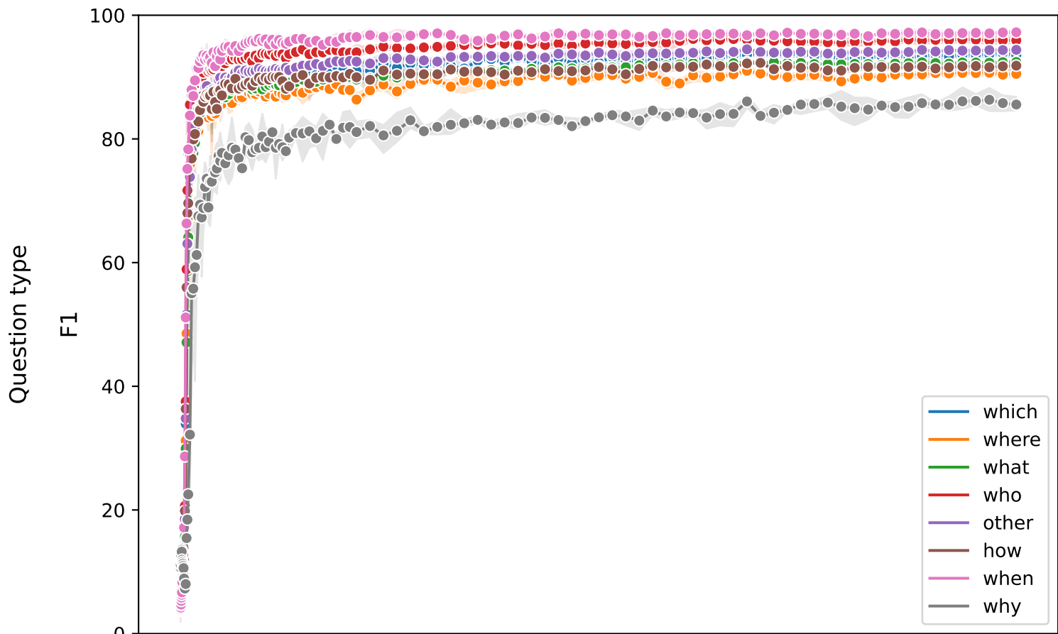
SQuAD 1.1
