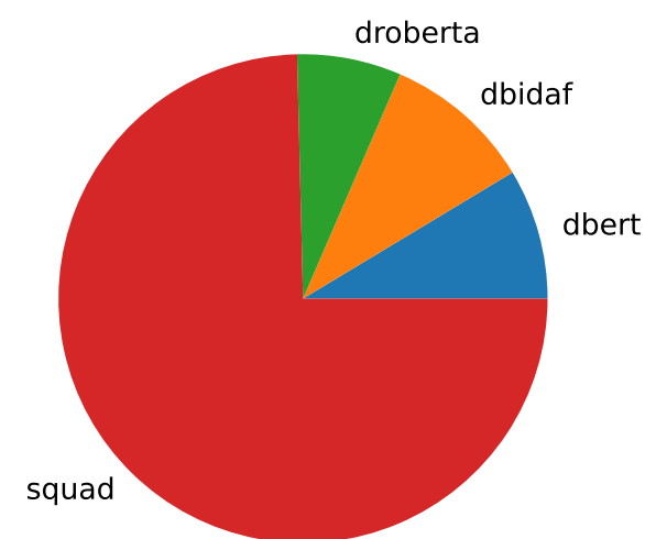
cluster 3 (n=2340)
