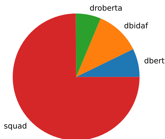
cluster 4 (n=984)
