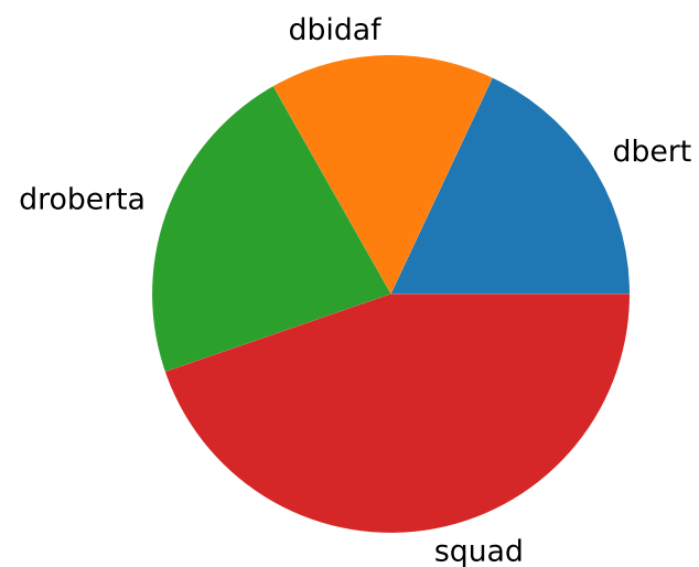
cluster 1 (n=1894)
