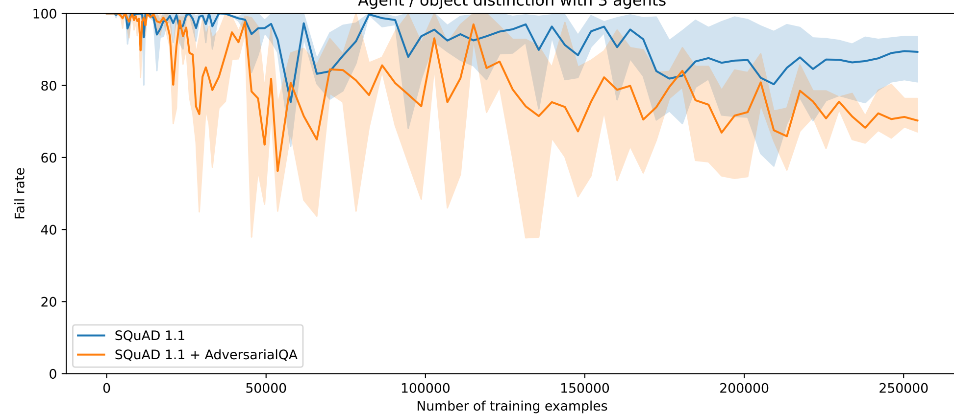
Agent / object distinction with 3 agents
