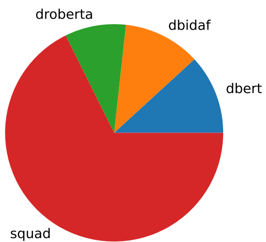
cluster 4 (n=1259)
