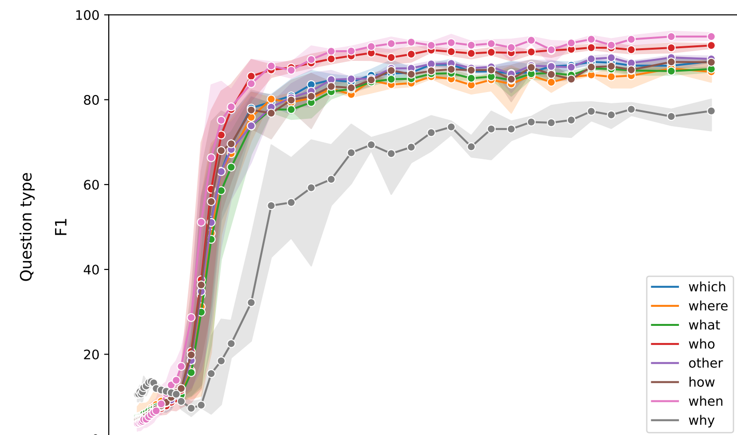
SQuAD 1.1
