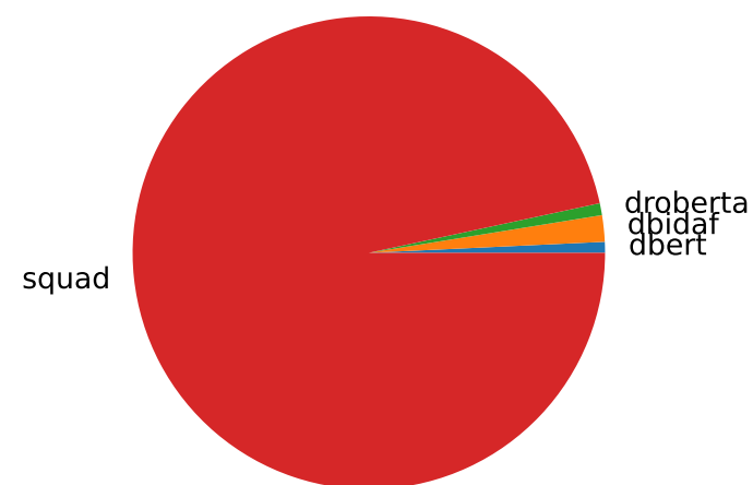
cluster 3 (n=2821)
