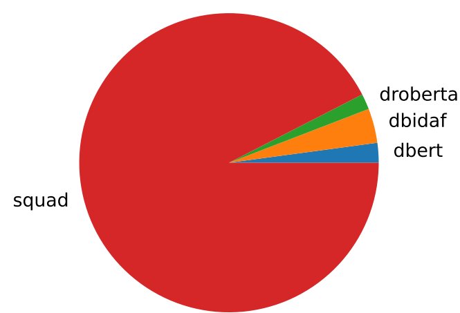
cluster 6 (n=2014)
