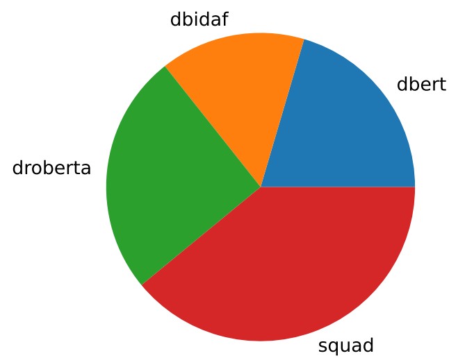
cluster 5 (n=533)
