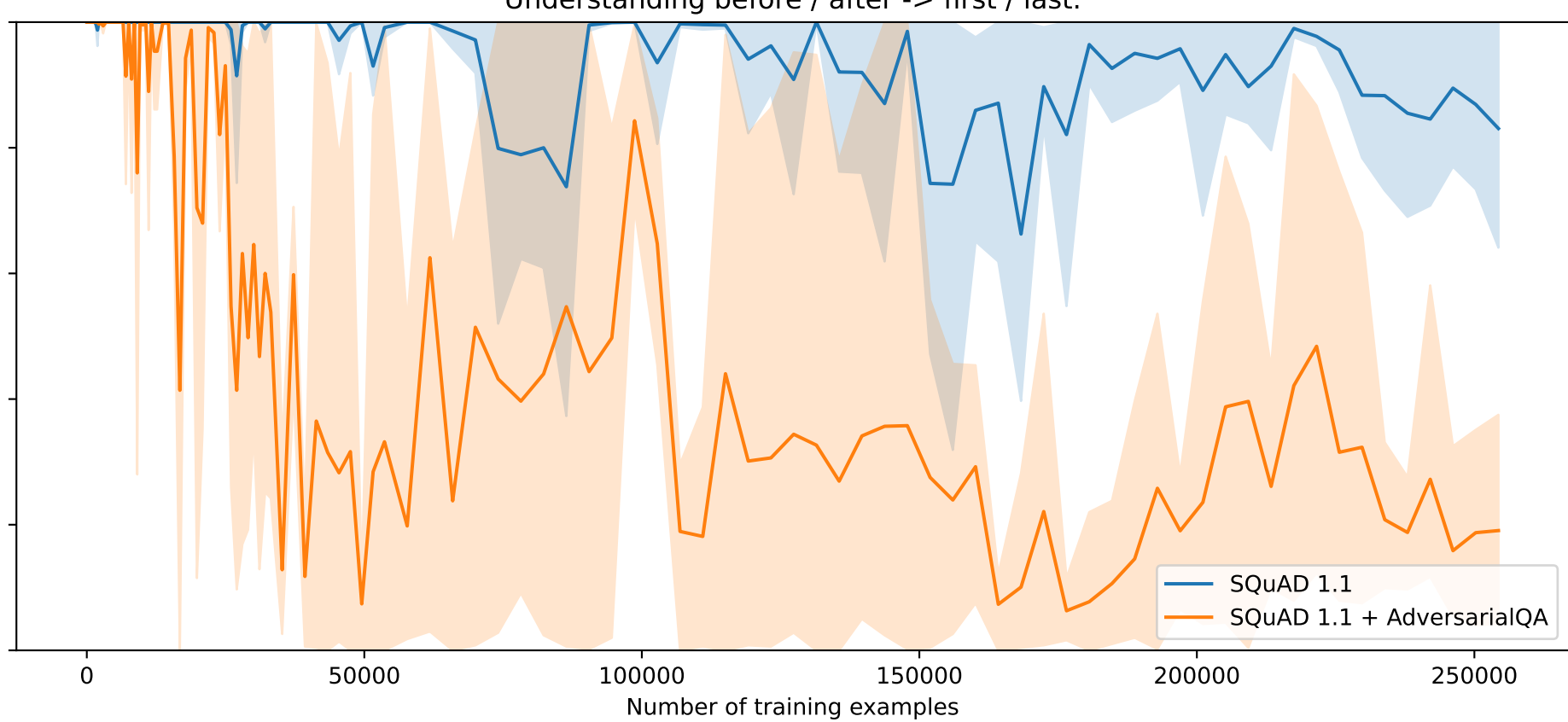
Understanding before / after -&gt; first / last.
