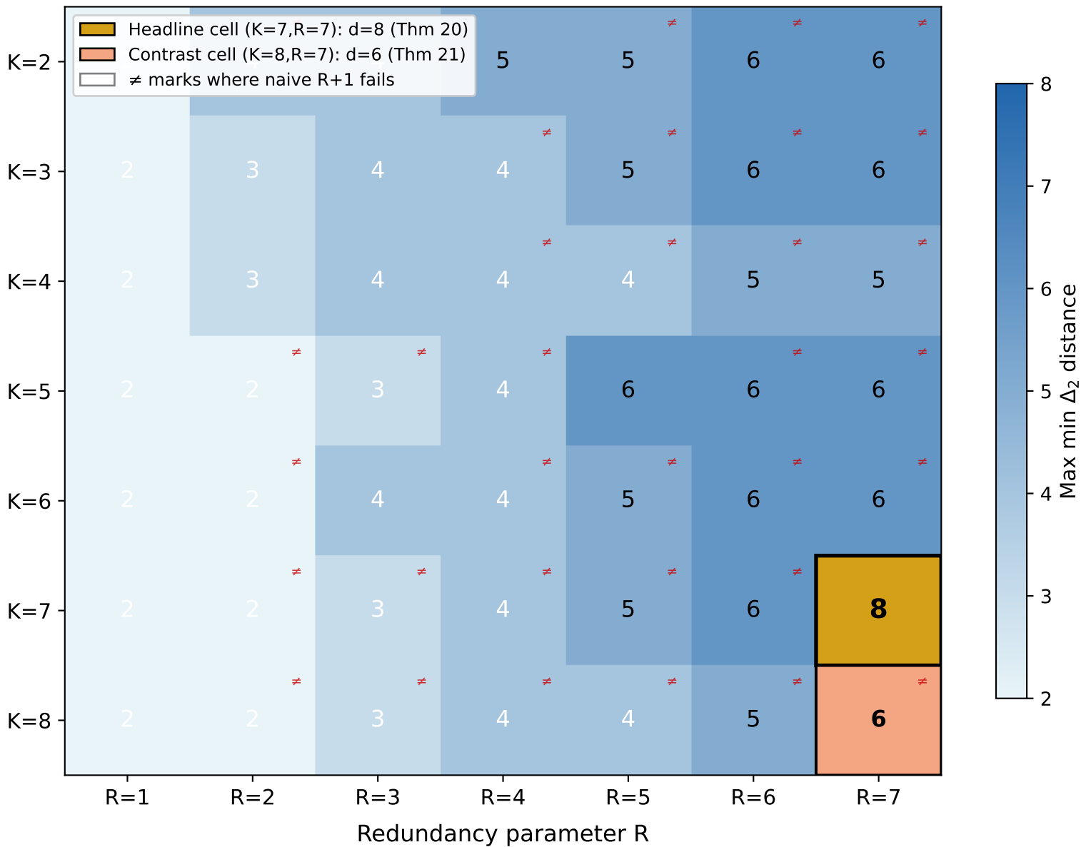
Phase diagram M_2(K, R) over \mathbb{Z}/4\mathbb{Z} under \Delta_2 metric (Theorem 19, SNS-THEORY-001)
