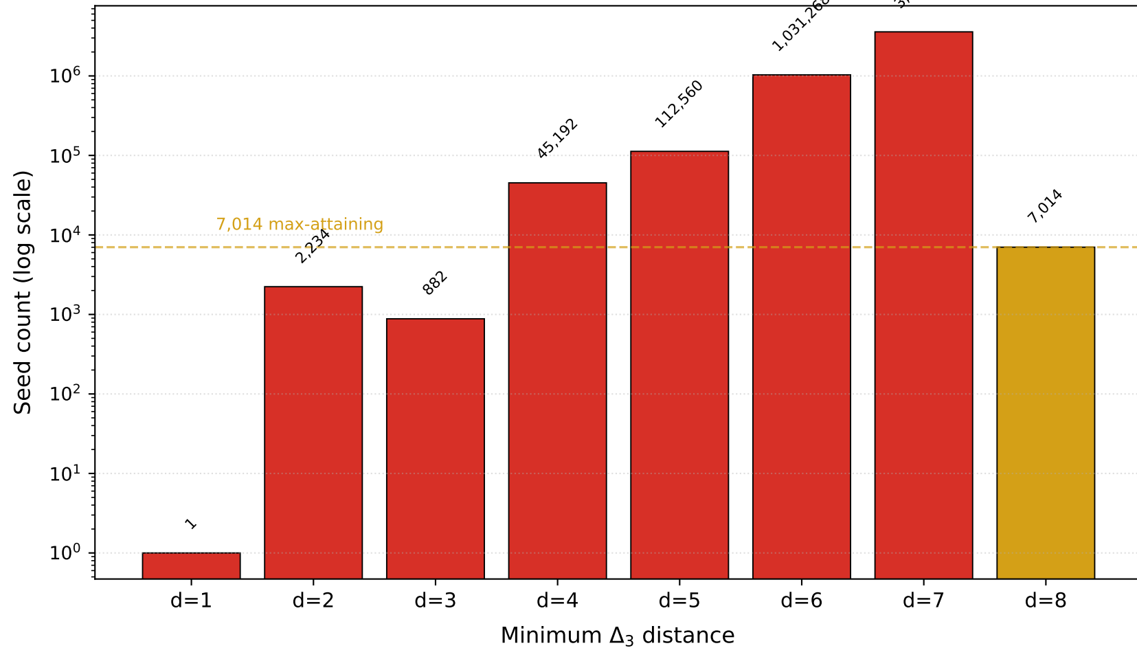
Distance histogram over (\mathbb{Z}/9\mathbb{Z})^7 , R = 7 (Theorem 24, SNS-THEORY-001)
