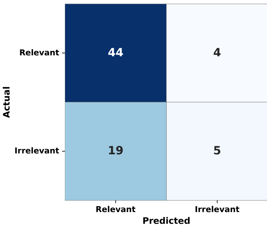
A) Pretrained Model: Relevance Classification
