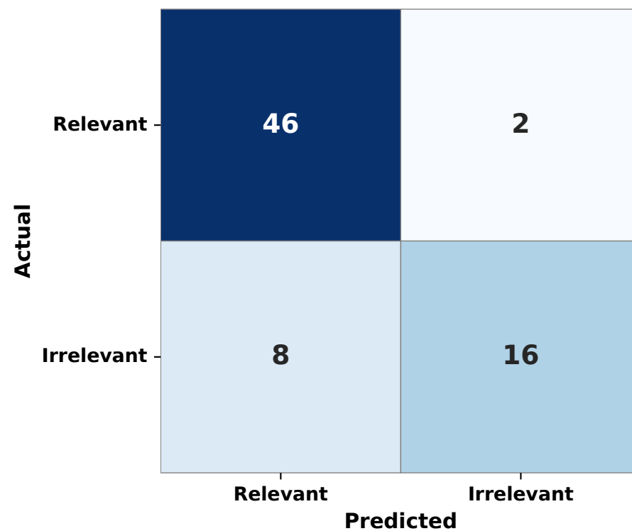
B) Fine-tuned Model: Relevance Classification
