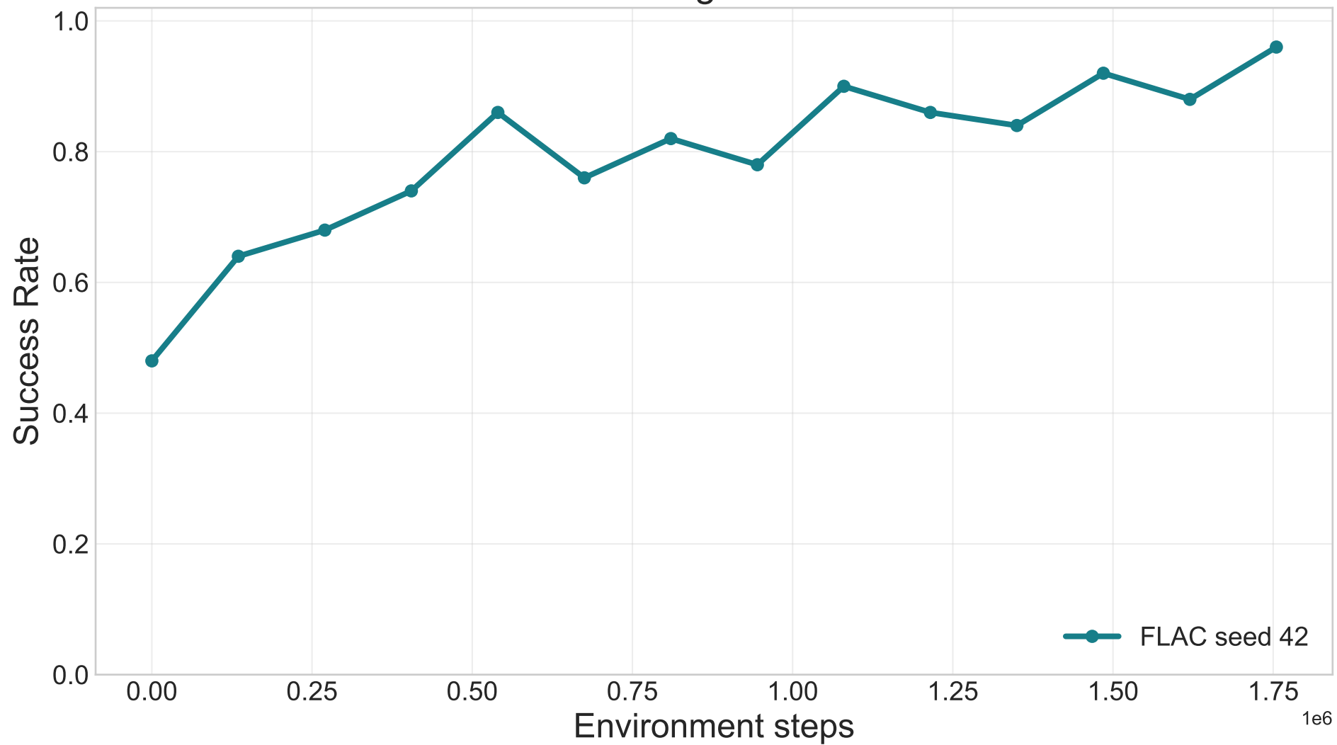
Robomimic can-img FLAC success rate
