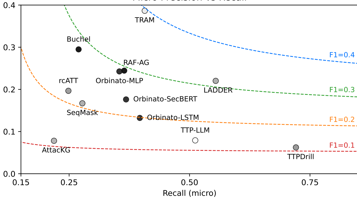
Micro Precision vs Recall
