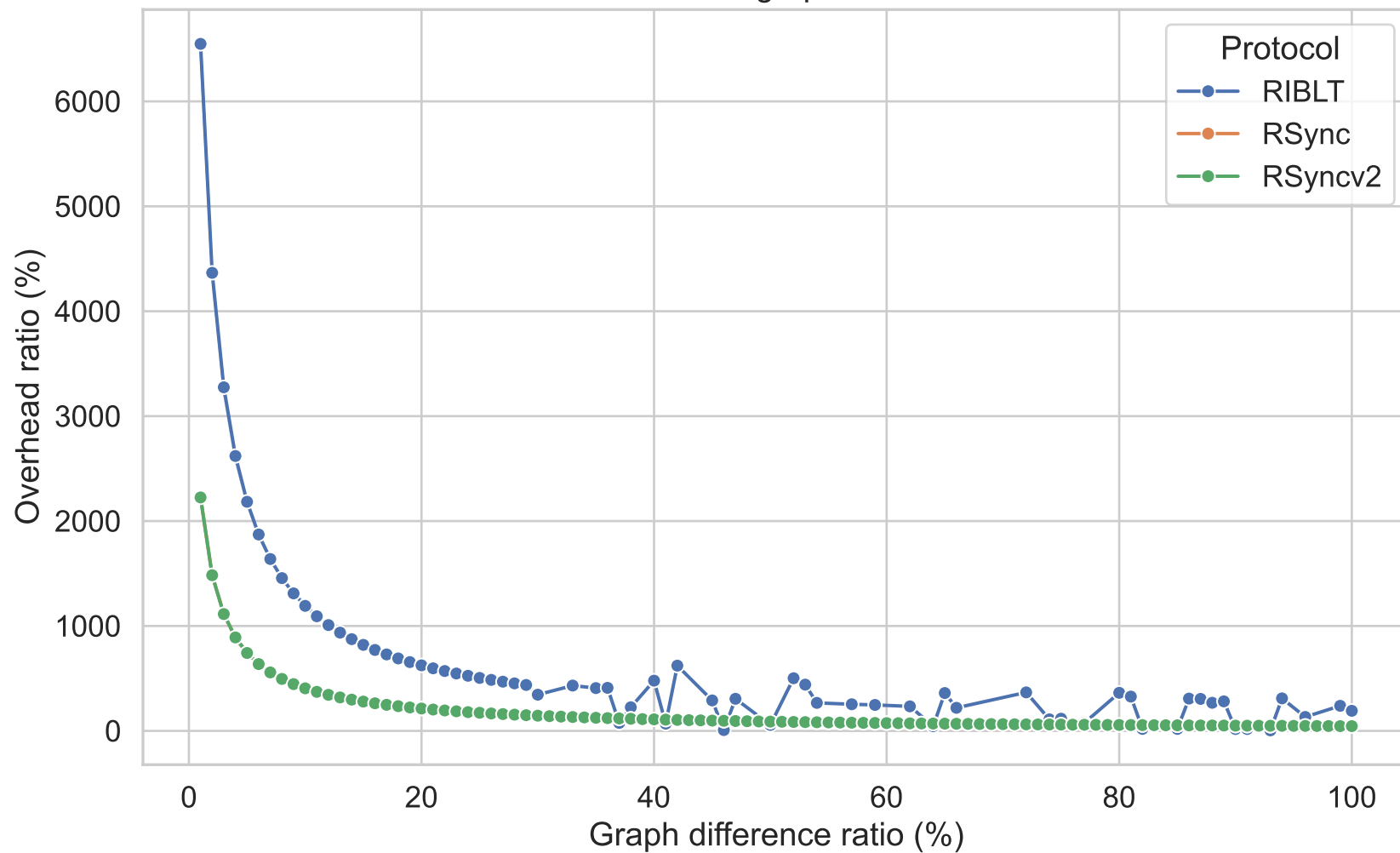
Overhead ratio vs graph difference ratio
