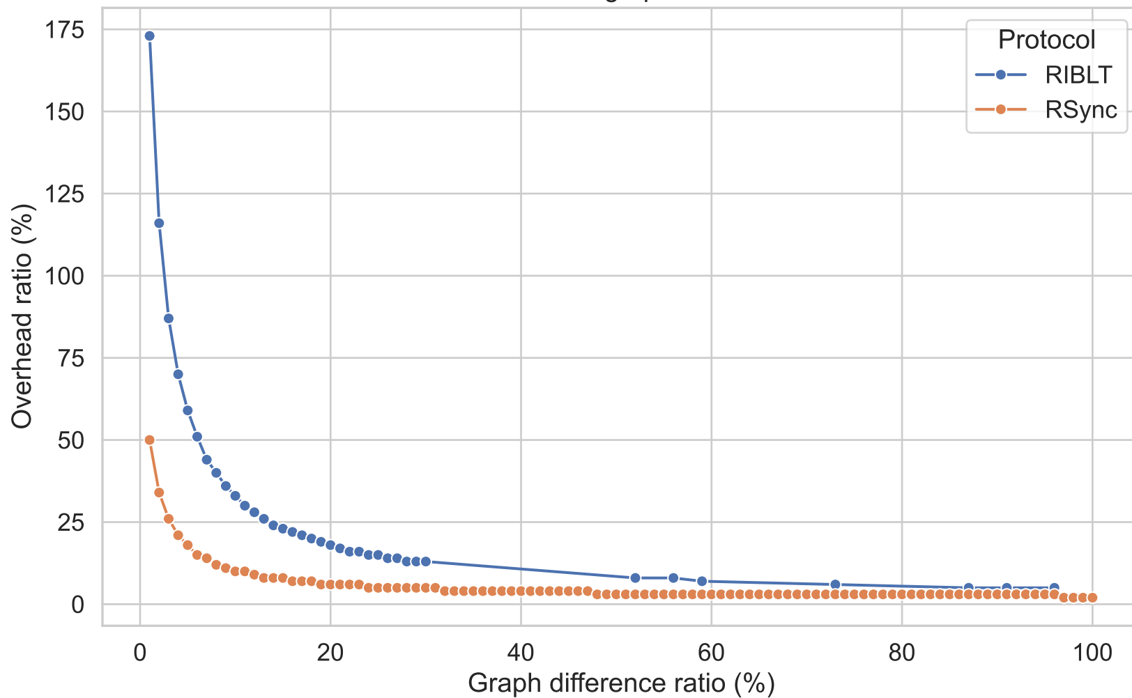
Overhead ratio vs graph difference ratio
