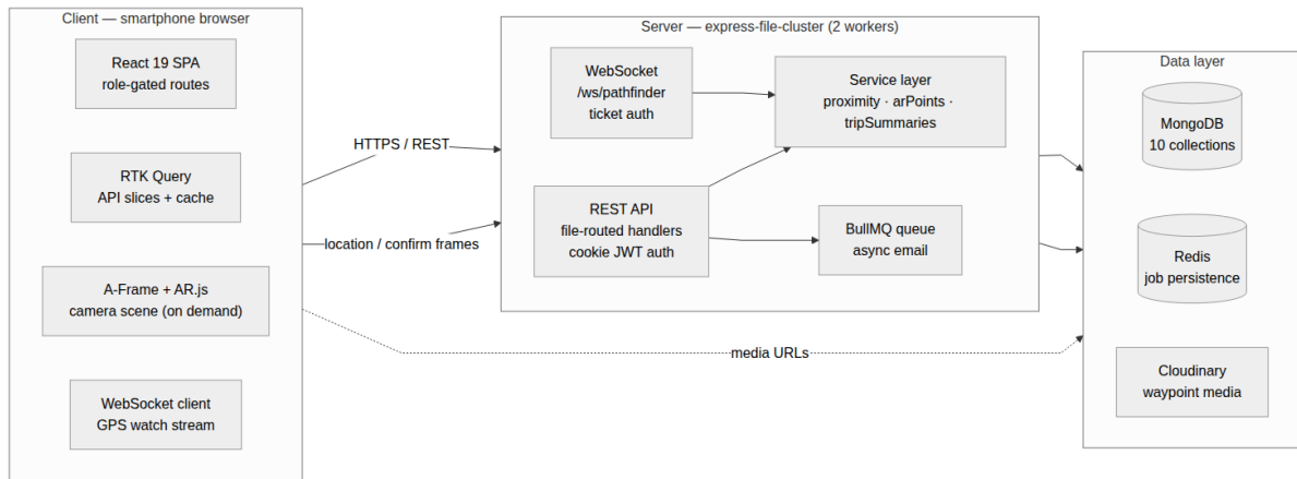
Figure 6.1: System architecture: client, server, and data layers.
