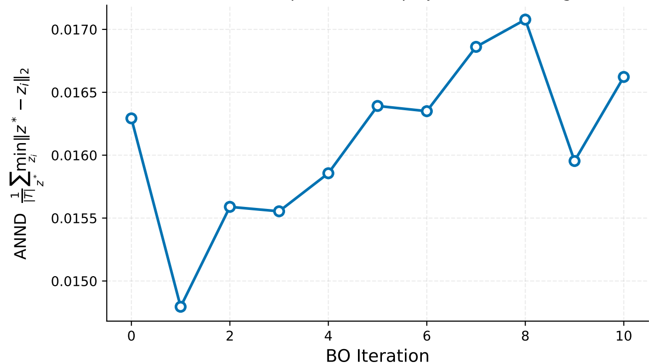
Average Nearest-Neighbor Distance (Test \rightarrow Train) in GP Feature Space (64-dim projected embeddings)
