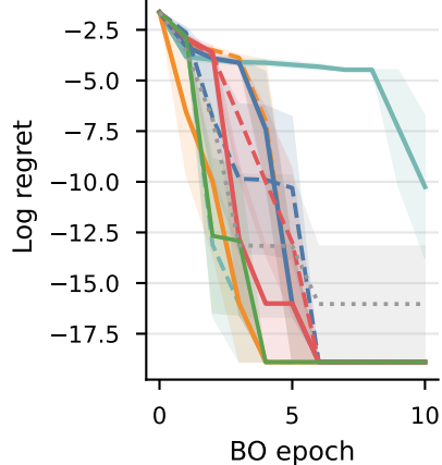
alpha-amylase / close to far
