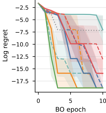
alpha-amylase / by mutation
