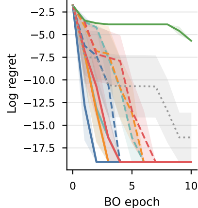
alpha-amylase / far to close
