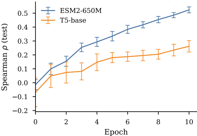
Spearman \rho on test split v/s BO epochs
