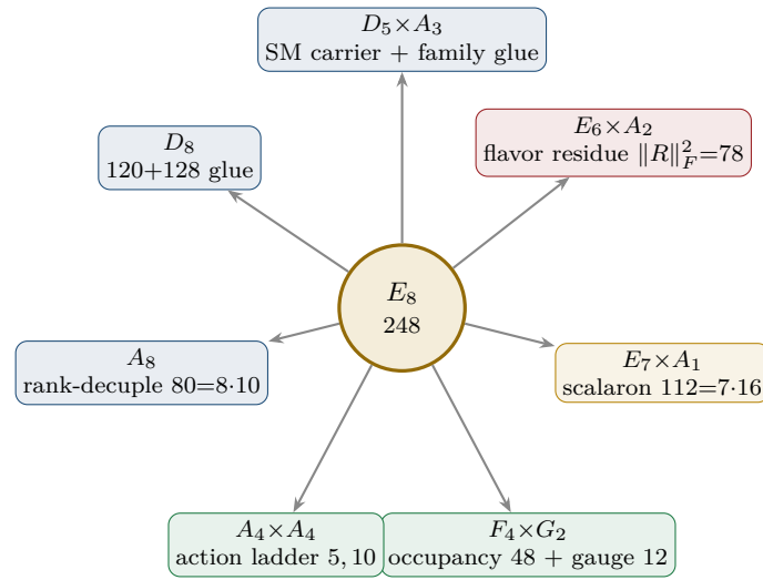
Figure 3: E_8 as an audit container: each maximal subalgebra projects one TFPT module. The discipline rule — every load-bearing number appears in \geq 1 projection — makes the structure falsifiable.
