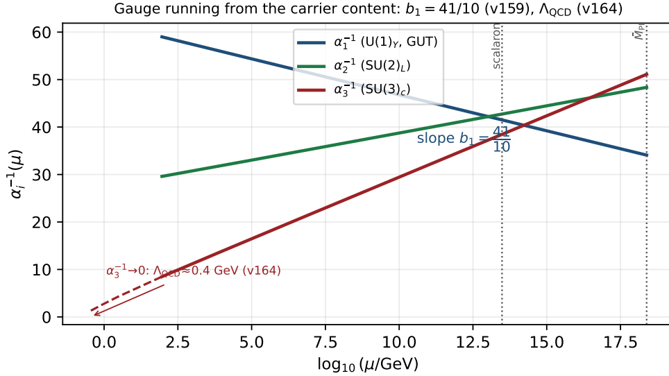
Figure 2: Gauge running from the carrier content (two-loop SM RGEs; the \beta -functions are confirmed by the external generator PyR@TE, [ verification/v159_pyrate_gauge_crosscheck.py ]). The U(1)_Y slope is the abelian index b_1 = 41/10 = 10^{-1}(g_{\text{car}}^{2g_{\text{car}}-2}+1) ; the strong coupling reaches confinement, \alpha_3^{-1} \rightarrow 0 at \Lambda_{\text{QCD}} \approx 0.4 GeV ([ verification/v164_qcd_scale.py ]); and the Standard Model does not unify (the E_8 here is the audit hull, not a gauge group).
