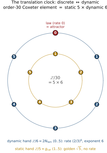
Figure 1: The translation clock ([ verification/v319_translation_clock.py ]): the discrete \leftrightarrow dynamic bridge is the order-30 Coxeter element read as two coprime hands. The dynamic hand ( \mathbb{Z}/6 = 2N_{\text{fam}} , outer, ticks 0.5) carries the recovery rate (2/3)^6 (exponent 6), with position 0 the conserved law (the attractor) and 1..5 the live phases; the static hand ( \mathbb{Z}/5 = g_{\text{car}} , inner, ticks 1..5) carries the golden \sqrt{5} and no rate. One full turn is \text{lcm}(5, 6) = 30 = h(E_8) . [E] (arithmetic) / [C] (the one-clock reading).
