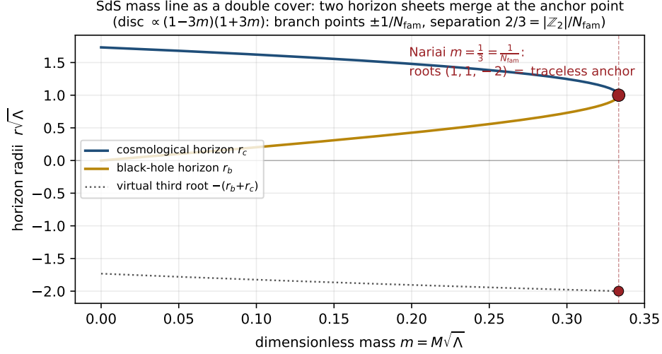
Figure 1: The SdS mass line as a double cover: black-hole and cosmological horizon sheets merge at the Nariai point m = 1/N_{\text{fam}} , where the three roots form the traceless anchor pattern (1, 1, -2) . [verification/v101_horizon_anchor.py]
