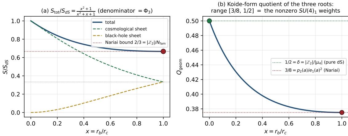
Figure 2: (a) Total SdS entropy interpolates from S_{dS} to the Narai bound \frac{2}{3}S_{dS} via (x^2+1)/\Phi_3(x) . (b) The Koide-form quotient of the three roots runs exactly over the nonzero SU(4)_1 weights [\frac{3}{8}, \frac{1}{2}] . [verification/v101_horizon_anchor.py]
