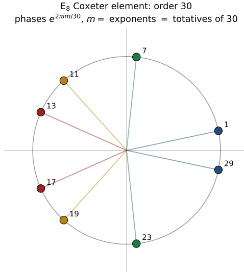
Figure 2: The E_8 Coxeter element (built from the Cartan matrix as c = s_1 \cdots s_8 ) has order exactly h(E_8) = 30 ; its eigenvalues are the primitive 30th roots e^{2\pi i m/30} with m the E_8 exponents \{1, 7, 11, 13, 17, 19, 23, 29\} , which are precisely the \varphi(30) = 8 totatives of 30. The phases pair as m + (30-m) = 30 into |\mu_4| = 4 invariant 2-planes. [L] ([verification/v55_coxeter_cycle.py])
