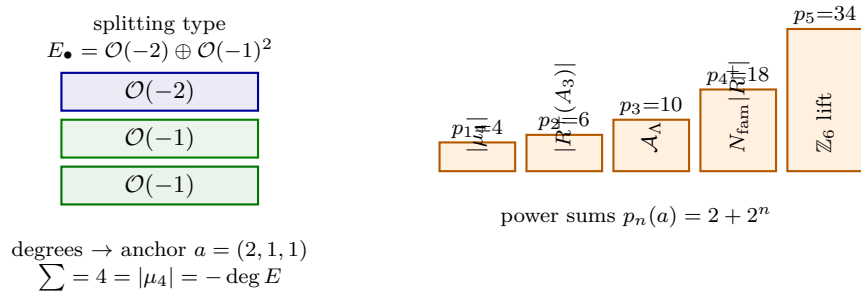
Figure 4: The (1, 1, 2) microcode. Left: the parabolic-stable splitting type \mathcal{O}(-2) \oplus \mathcal{O}(-1)^2 whose degrees are the anchor. Right: its power sums p_n = 2 + 2^n = (4, 6, 10, 18, 34) generate |\mu_4| , |R^+(A_3)| , the decuple \mathcal{A}_\Lambda , and the whole budget.
