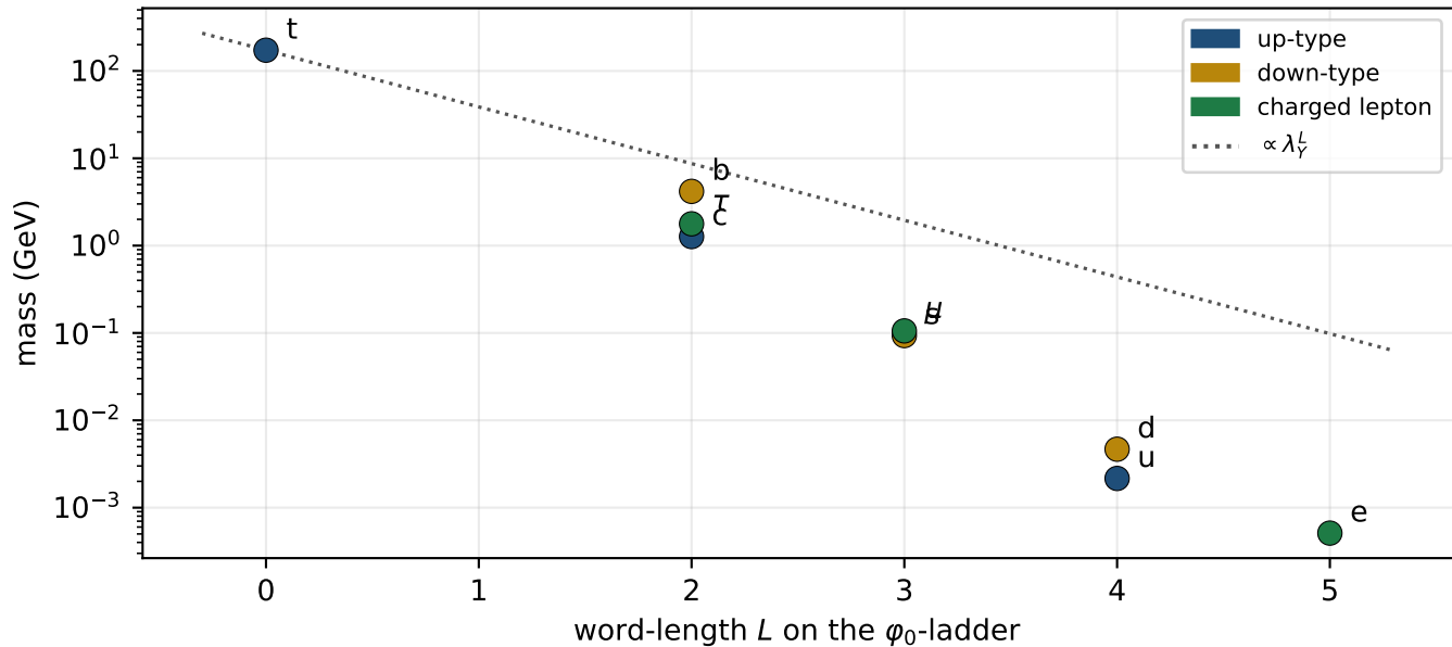
Mass ladder: nine fermions on one \varphi_0 -ladder
