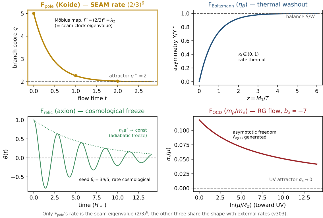
Figure 4: The discrete→dynamic lens on F_{\text{transfer}} ([ verification/v303_ftransfer_dynamics.py ]). All four transfer instances share one shape — a gapped, positivity-preserving relaxation to a unique attractor, the same Perron-Frobenius / H-theorem / RG-fixed-point structure as the main-branch update m \leftarrow (A+2I)/4m \rightarrow the E_8 marks. Only F_{\text{pole}} (Koide, gold) runs it at the seam rate: its Möbius multiplier is F'=(2/3)^6=\lambda_2 , the seam-clock subleading eigenvalue. F_{\text{Boltzmann}} ( \eta_B , thermal washout), F_{\text{relic}} (axion, cosmological freeze) and F_{\text{QCD}} ( m_p/m_e , the RG flow to the Gaussian UV fixed point with the carrier b_3=-7 ) share the shape with external rates. So F_{\text{transfer}} is the readout end of the one principle, not a bolt-on; the theory’s simplicity is preserved because the external rates are honestly fenced (v187), not reduced to the seam.
