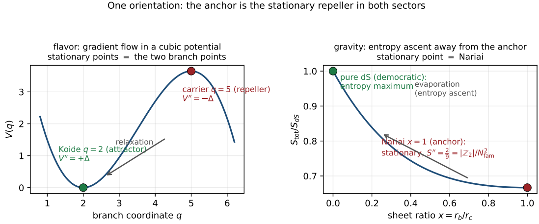
Figure 2: One orientation, two sectors: the anchor configuration is the stationary repeller of the natural functional — the cubic flavor potential (curvatures \pm\Delta ) and the SdS entropy (curvature 2/9 = |\mathbb{Z}_2|/N_{\text{fam}}^2 ). [E] ([ verification/v102_seam_orientation.py ]); the common-principle reading stays [C].
