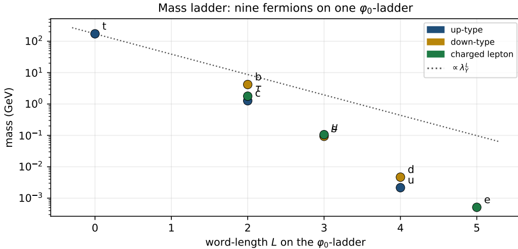
Figure 1: Mass ladder (data plot, verification/make_figures.py). The nine charged fermions (PDG masses) plotted against their word-length L on the \varphi_0^{\text{ret}} -ladder, coloured by sector; the dotted line is the geometric reference \propto \lambda_Y^L with \lambda_Y = \sqrt{\varphi_0^{\text{ret}}(1 - \varphi_0^{\text{ret}})} . The whole five-order hierarchy is one ladder.
