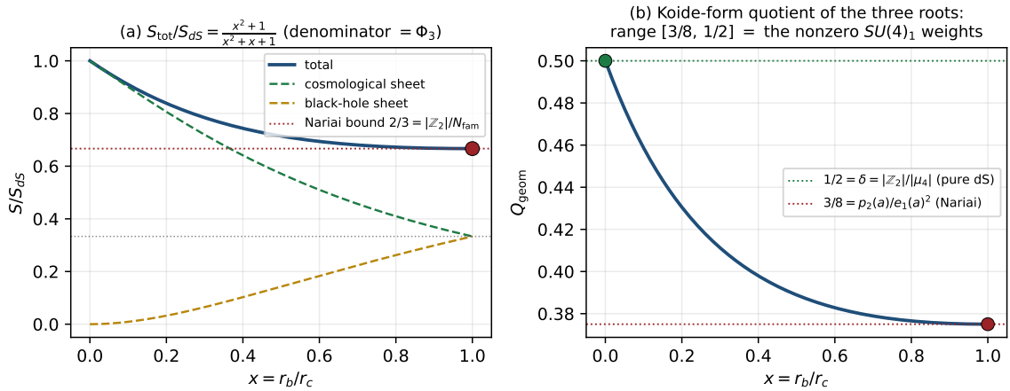
Figure 2: (a) Total SdS entropy interpolates from S_{\text{dS}} to the Nariai bound \frac{2}{3}S_{\text{dS}} via (x^2+1)/\Phi_3(x) . (b) The Koide-form quotient of the three roots runs exactly over the nonzero SU(4)_1 weights [\frac{3}{8}, \frac{1}{2}] . [ verification/v101_horizon_anchor.py ]
