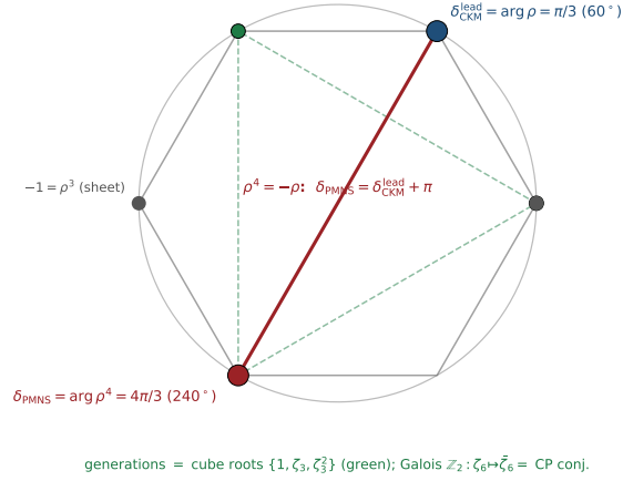
Figure 2: The Galois CP lock ([ verification/v320_galois_cp_relation.py ]): both leading CP phases are powers of the one hexagonal unit \rho = \zeta_6 — \delta_{\text{CKM}}^{\text{lead}} = \arg \rho = \pi/3 (blue) and \delta_{\text{PMNS}} = \arg \rho^4 = 4\pi/3 (red) — locked by \rho^4 = -\rho to \delta_{\text{PMNS}} = \delta_{\text{CKM}}^{\text{lead}} + \pi . The three generations are the even vertices (cube roots \{1, \zeta_3, \zeta_3^2\} , green, §4); the family Galois \mathbb{Z}_2 ( \zeta_6 \mapsto \bar{\zeta}_6 ) is CP conjugation. [E] (relation) / [C] (phase identification) / [X] (kill test).
