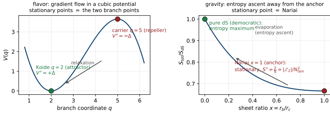
Figure 4: One orientation, two sectors: the anchor configuration is the stationary repeller of the natural functional — the cubic flavor potential (curvatures \pm\Delta ) and the SdS entropy (curvature 2/9 = |\mathbb{Z}_2|/N_{\text{fam}}^2 ). [E] ([verification/v102_seam_orientation.py]); the common-principle reading stays [C].
