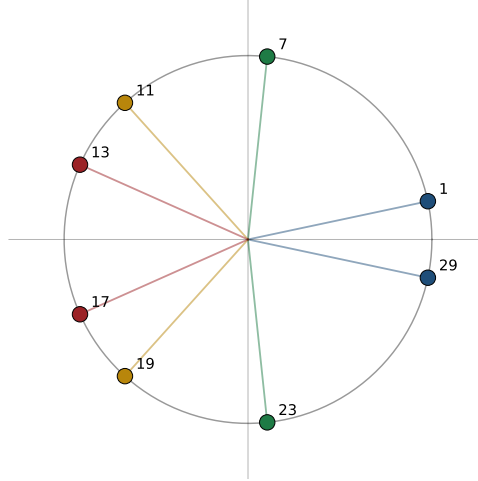
E_8 Coxeter element: order 30 phases e^{2\pi im/30} , m = \text{exponents} = \text{totatives of } 30
