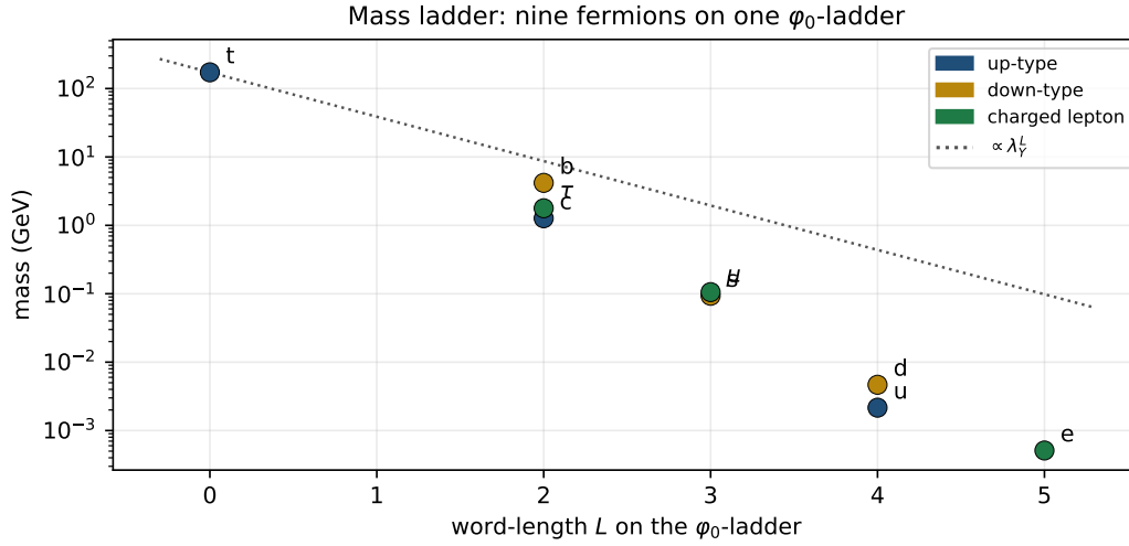
Figure 1: Mass ladder (data plot, verification/make_figures.py ). The nine charged fermions (PDG masses) plotted against their word-length L on the \varphi_0^{\text{ret}} -ladder, coloured by sector; the dotted line is the geometric reference \propto \lambda_Y^L with \lambda_Y = \sqrt{\varphi_0^{\text{ret}}(1 - \varphi_0^{\text{ret}})} . The whole five-order hierarchy is one ladder.
