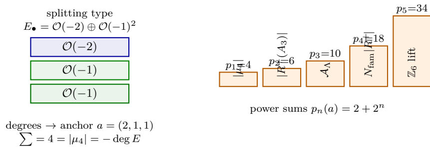
Figure 3: The (1, 1, 2) microcode. Left: the parabolic-stable splitting type \mathcal{O}(-2) \oplus \mathcal{O}(-1)^2 whose degrees are the anchor. Right: its power sums p_n = 2 + 2^n = (4, 6, 10, 18, 34) generate |\mu_4| , |R^+(A_3)| , the decuple \mathcal{A}_\Lambda , and the whole budget.
