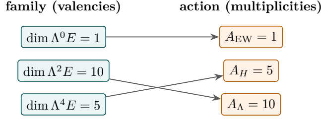
Figure 1: Exterior–Action duality. The Standard-Model family is the valency side of the even Hamming scheme on the five-slot code; the cosmological action ladder is its spectral (multiplicity) side. The \Lambda (pair) sector \Lambda^2 E has dimension \binom{5}{2} = 10 , the origin of the decuple exponent.
