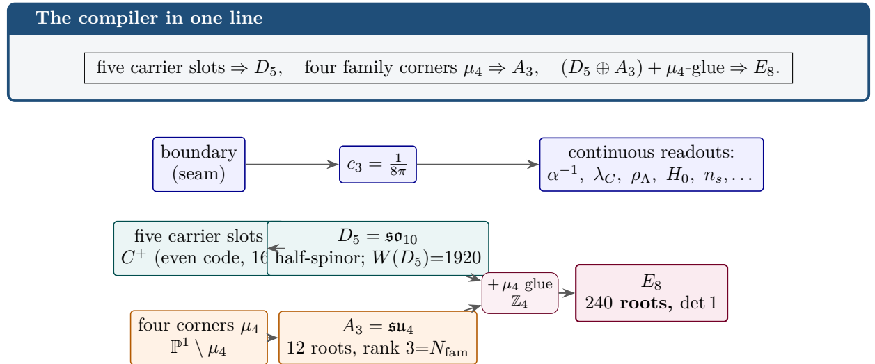
Figure 2: The explanation hierarchy. The boundary fixes the seam seed c_3 ; the five-slot even carrier code is the D_5 half-spinor; the four punctures \mu_4 give A_3 ; their common \mathbb{Z}_4 discriminant ( \mu_4 ) glues D_5 \oplus A_3 into the unimodular E_8 . E_8 is the closure , not the input; c_3 dresses the continuous observables.
