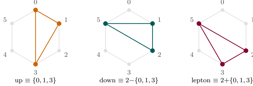
Figure 5: Flavor transport on the hexagon C_6 = Z_6 = |R^+(A_3)| . The unique distinct-distance triple \{0, 1, 3\} (cyclic distances \{1, 2, 3\} ) and its D_6 orbit give the three sectors' residues mod 6; the total \sum L = 40 = |R(D_5)| and the first-generation +6 winding come from the carrier.
