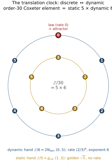
Figure 1: The translation clock ([verification/v319_translation_clock.py]): the discrete↔dynamic bridge is the order-30 Coxeter element read as two coprime hands. The dynamic hand ( Z/6 = 2N_{\text{fam}} , outer, ticks 0..5) carries the recovery rate (2/3)^6 (exponent 6), with position 0 the conserved law (the attractor) and 1..5 the live phases; the static hand ( Z/5 = g_{\text{car}} , inner, ticks 1..5) carries the golden \sqrt{5} and no rate. One full turn is \text{lcm}(5, 6) = 30 = h(E_8) . [E] (arithmetic) / [C] (the one-clock reading).
