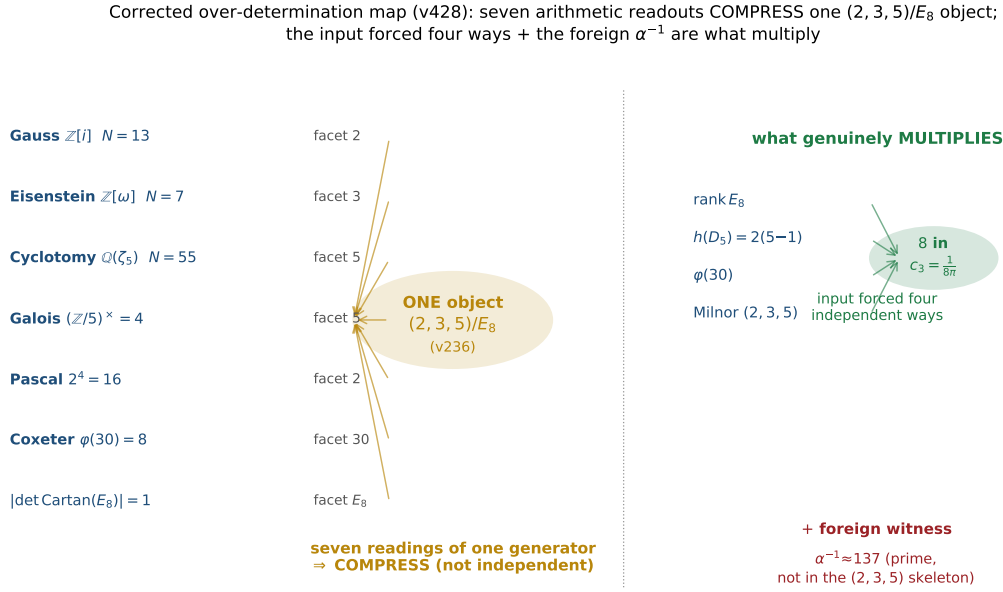
Figure 3: The corrected over-determination map ([ verification/v428_overdet_reclass.py ]): the seven arithmetic readouts are facets of one (2, 3, 5)/E_8 object (a compression gain, like the anchor), so they do not multiply; what genuinely multiplies is the input forced four independent ways (the “8”) plus the foreign witness \alpha^{-1} \approx 137 . The disjoint pieces give an unconditional floor \sim 10^{-10} ([ verification/v432_overdet_floor.py ]), \sim 20 orders above the conditional 10^{-30.7} ; hardened to an assumption-minimal counting floor 1/94\,500 \approx 4.40\sigma ([ verification/v436_overdet_floor2.py ]) that drops every subjective chance assignment and a monotone concession ladder ( 30.7 \rightarrow 25.8 \rightarrow 4.98 dex) that keeps the “not chance” verdict at the most adversarial rung.
