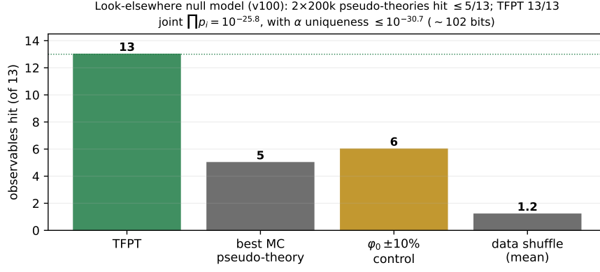
Figure 4: The look-elsewhere null model ([ verification/v100_numerology_null_mc.py ]): Monte-Carlo pseudo-theories hit at most 5/13 where TFPT hits 13/13; the power controls ( \phi_0^{\text{ret}} \pm 10\% , data shuffle) confirm the test is non-vacuous.
