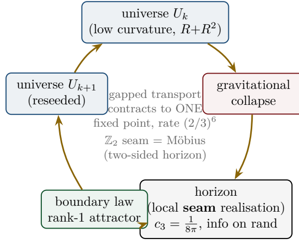
Figure 6: [C] The cyclic reading. Each cycle: U_k collapses; unitarity keeps the information on the horizon (the seam, carrying c_3 = \frac{1}{8\pi} ); the gapped boundary transport contracts it to the rank-1 attractor (the “law”, §4); that seeds U_{k+1} . The \mathbb{Z}_2 = g_{\text{car}} - N_{\text{fam}} sheet parity is the Möbius/two-sided (thermofield-double) gluing across the horizon. Realized constants = the attractor’s fixed point, hence parameter-free.
