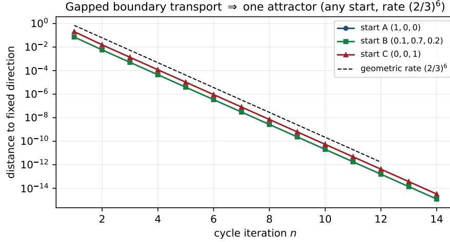
Figure 5: The transport spectrum \{1, (2/3)^6, (1/3)^6\} has spectral gap \Delta = -\log(2/3)^6 = 2.4328 > 0 . By Perron–Frobenius the operator has a unique dominant eigenvector; iterating from any start converges to the same fixed direction at the geometric rate \lambda_2/\lambda_1 = (2/3)^6 — the same \lambda_2 that fixes flavor and horizon recovery. [E] ([verification/v56_unique_attractor.py])
