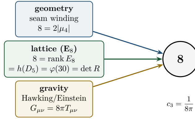
Figure 2: The seam denominator 8 is fixed three independent ways. If the seam is a horizon, the gravitational 8\pi (Hawking temperature T_H = c_3/M , Einstein G_{\mu\nu} = 8\pi T_{\mu\nu} ) forces c_3 ; it must then coincide with the geometric 2|\mu_4| (Gauss–Bonnet seam winding) and the lattice rank E_8 . All three give 8. [E] ([verification/v54_seam_horizon_keystones.py])
