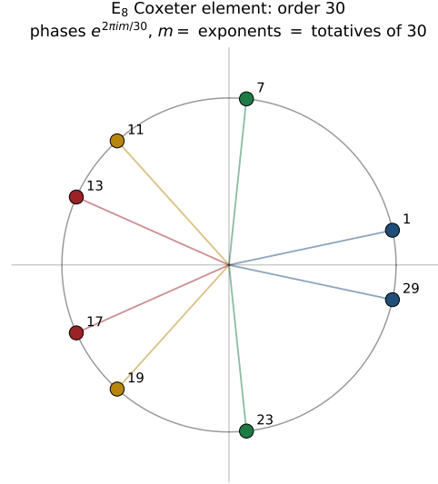
Figure 4: The E_8 Coxeter element (built from the Cartan matrix as c = s_1 \cdots s_8 ) has order exactly h(E_8) = 30 ; its eigenvalues are the primitive 30th roots e^{2\pi im/30} with m the E_8 exponents \{1, 7, 11, 13, 17, 19, 23, 29\} , which are precisely the \varphi(30) = 8 totatives of 30. The phases pair as m + (30 - m) = 30 into |\mu_4| = 4 invariant 2-planes. [E] ([verification/v55_coxeter_cycle.py])
