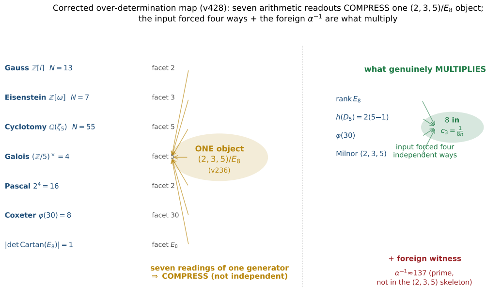
Figure 3: The corrected over-determination map ([verification/v428_overdet_reclass.py]): the seven arithmetic readouts are facets of one (2, 3, 5)/E_8 object (a compression gain, like the anchor), so they do not multiply; what genuinely multiplies is the input forced four independent ways (the “8”) plus the foreign witness \alpha^{-1} \approx 137 .
