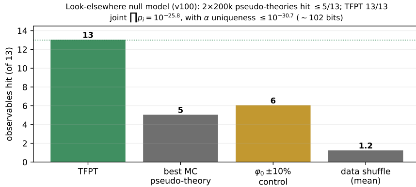
Figure 4: The look-elsewhere null model ([ verification/v100_numerology_null_mc.py ): Monte-Carlo pseudo-theories hit at most 5/13 where TFPT hits 13/13; the power controls ( \varphi_0^{\text{ret}} \pm 10\% , data shuffle) confirm the test is non-vacuous.
