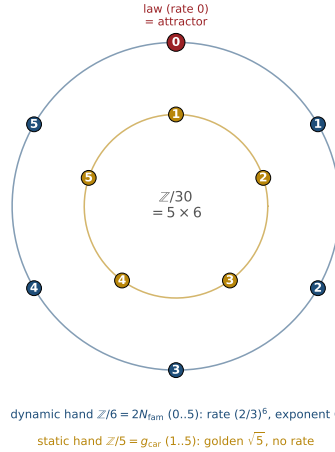
Figure 1: The translation clock ([verification/v319_translation_clock.py]): the discrete \leftrightarrow dynamic bridge is the order-30 Coxeter element read as two coprime hands. The dynamic hand ( \mathbb{Z}/6 = 2N_{\text{fam}} , outer, ticks 0..5) carries the recovery rate (2/3)^6 (exponent 6), with position 0 the conserved law (the attractor) and 1..5 the live phases; the static hand ( \mathbb{Z}/5 = g_{\text{car}} , inner, ticks 1..5) carries the golden \sqrt{5} and no rate. One full turn is \text{lcm}(5,6) = 30 = h(E_8) . [E] (arithmetic) / [C] (the one-clock reading).
