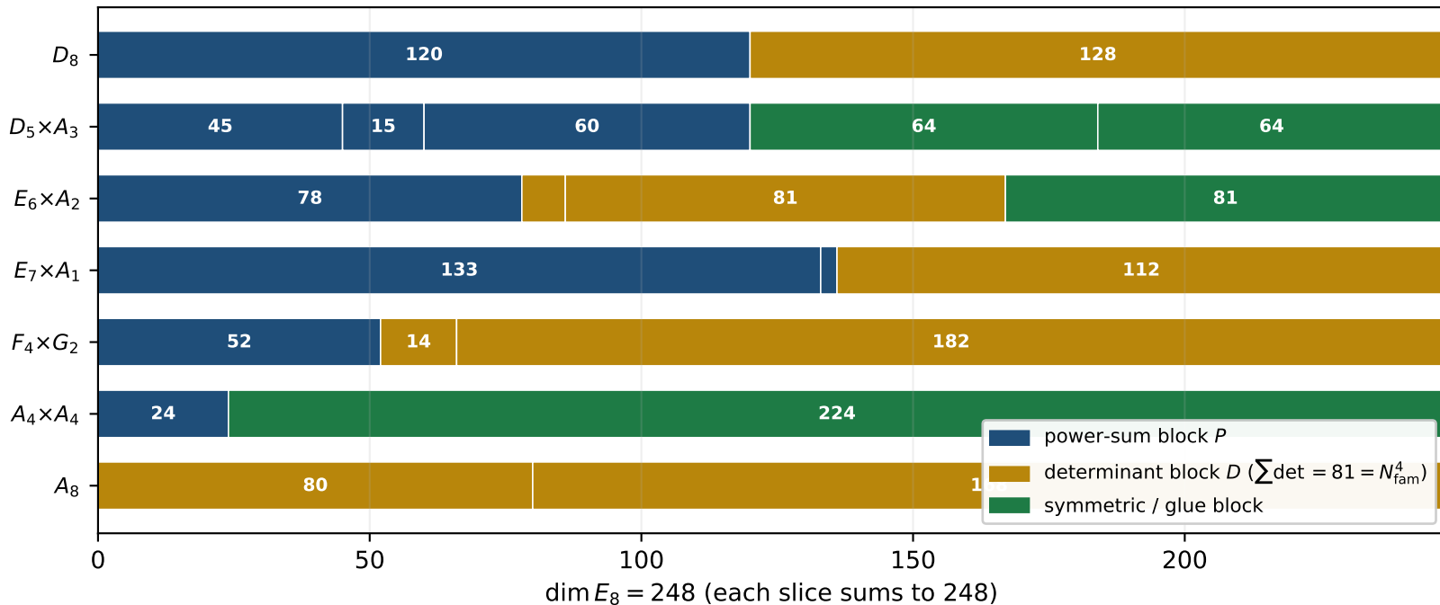
E_8 slice compression: seven slices, two alphabets P = (3, 4, 6, 10) , D = (3, 4, 8, 14, 20, 32)
