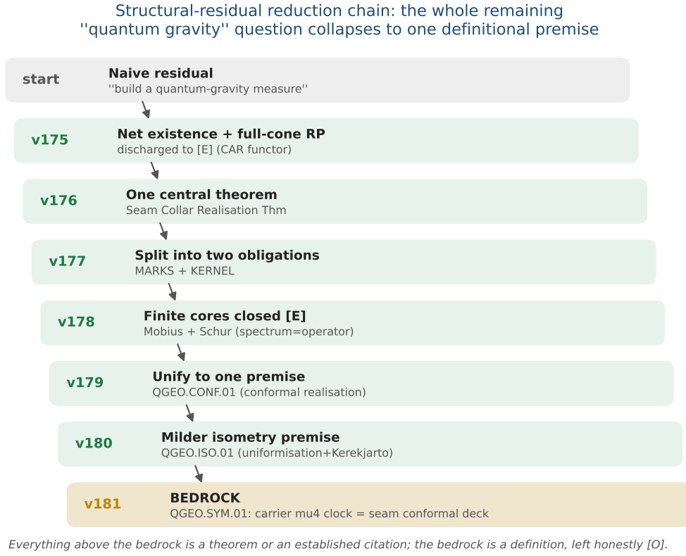
Figure 1: The structural-residual reduction chain (v175–v181). The naive “build a quantum-gravity measure” shrinks, one machine-checked step at a time, to a single definitional geometric premise QGE0.SYM.01 (the carrier \mu_4 clock is the seam’s conformal deck). Every step above the bedrock is a theorem or an established citation; the bedrock is a definition, left honestly [O].
