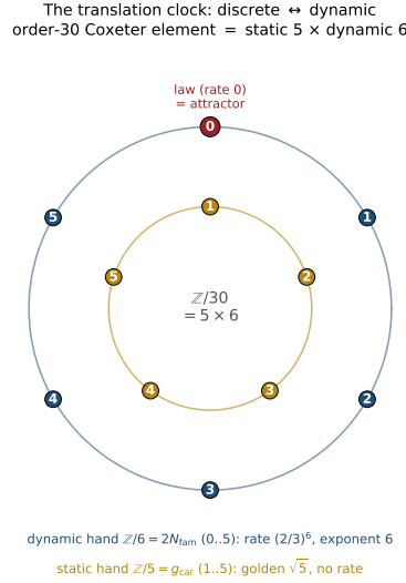
Figure 1: The translation clock ([verification/v319_translation_clock.py]): the discrete↔dynamic bridge is the order-30 Coxeter element read as two coprime hands. The dynamic hand ( \mathbb{Z}/6 = 2N_{\text{fam}} , outer, ticks 0..5) carries the recovery rate (2/3)^6 (exponent 6), with position 0 the conserved law (the attractor) and 1..5 the live phases; the static hand ( \mathbb{Z}/5 = g_{\text{car}} , inner, ticks 1..5) carries the golden \sqrt{5} and no rate. One full turn is \text{lcm}(5, 6) = 30 = h(E_8) . [E] (arithmetic) / [C] (the one-clock reading).
