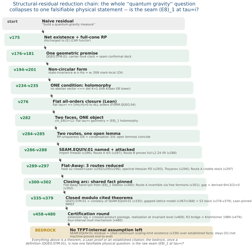
Figure 3: The structural-residual reduction chain ( v175 \rightarrow the certification round). The naive “build a quantum-gravity measure” shrinks, one machine-checked step at a time, from a vague measure to one falsifiable physical statement — is the raw seam (E_8)_1 at \tau = i ? (SEAM.EQUIV.01; its conformal-deck face QGEO.SYM.01 is a corollary, v335). The closing arc ( v276 – v302 ) pins the shared fact and derives the gap 6\ln(3/2) > 0 ; the certification round discharges the extension leg to the crossed-product package (v469), the R3 graph→geometry bridge to Kronheimer 1989 (v479) and exhibits the four-interval \mu_4 mechanism (v480). Every step above the bedrock is a theorem, a Lean proof or an established citation; the residual — the cited continuum scaling-limit existence (v336) — stays honestly [O].
