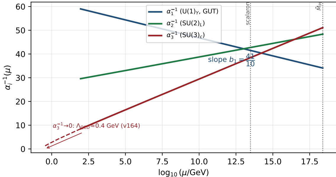
Gauge running from the carrier content: b_1 = 41/10 (v159), \Lambda_{\text{QCD}} (v164)
