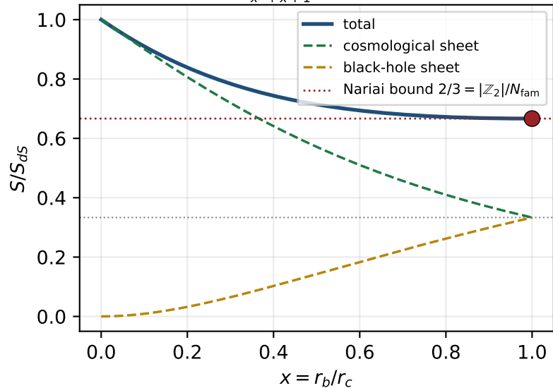
(a) S_{\text{tot}}/S_{\text{dS}} = \frac{x^2+1}{x^2+x+1} (denominator = \Phi_3 )
