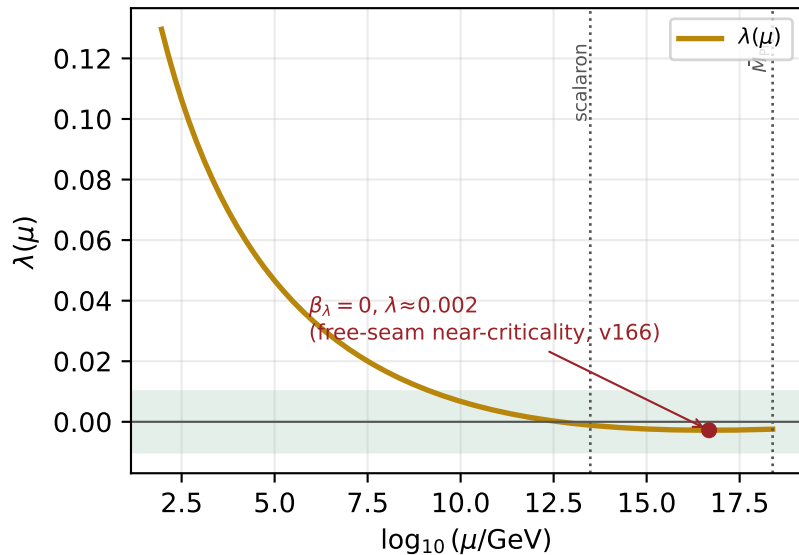
Higgs quartic: free seam \Rightarrow \lambda(\bar{M}_{\text{Pl}}) \approx 0
