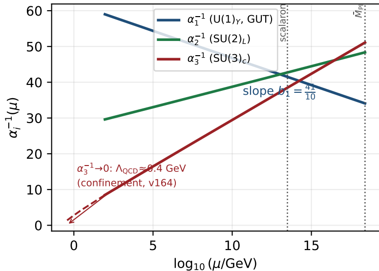
Gauge running: b_1 = 41/10 , confinement, no SM unification
