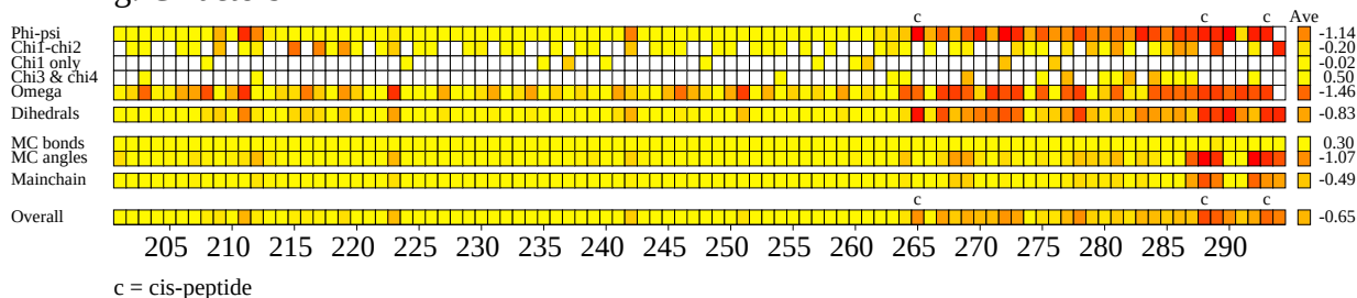
g. G-factors
