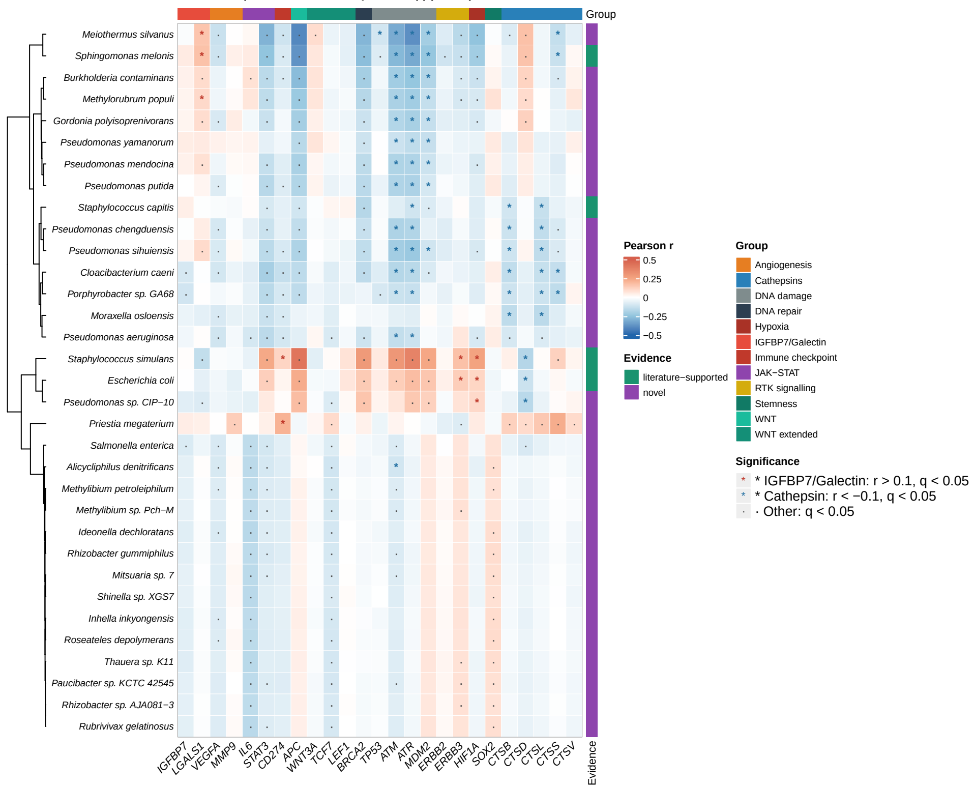
Breast invasive carcinoma (BRCA) Pearson r | Bacteria × Gene Expression | |r| > 0.1 | n = 1095 tumours
