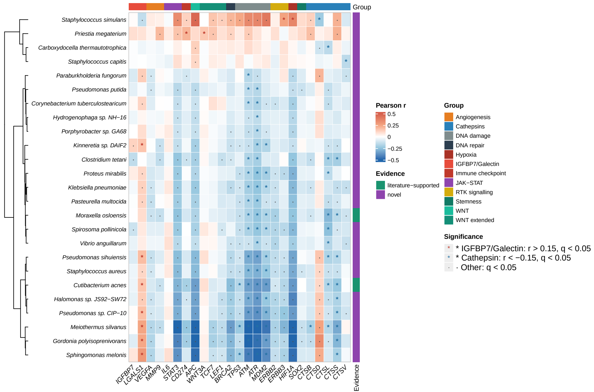
Prostate adenocarcinoma (PRAD) Pearson r | Bacteria × Gene Expression | |r| > 0.15 | n = 497 tumours
