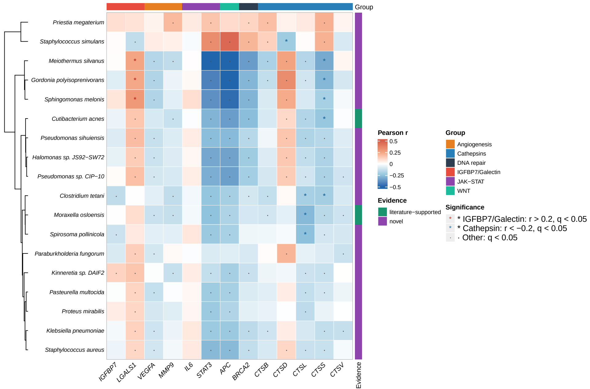
Prostate adenocarcinoma (PRAD) Pearson r | Bacteria × Gene Expression | |r| > 0.2 | n = 497 tumours
