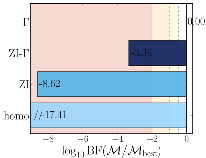
Kills: aggregate \log_{10} BF across conditions
