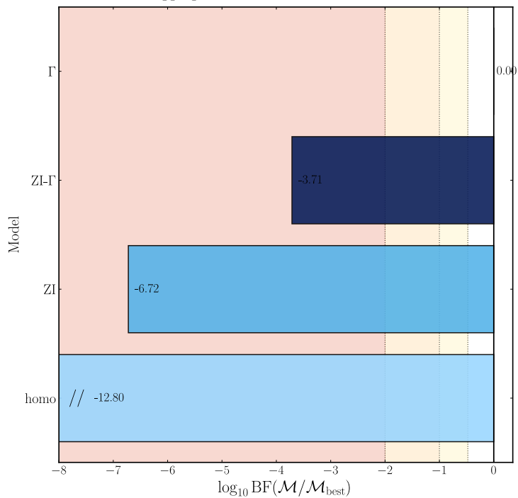
Aggregate across three conditions: kills
