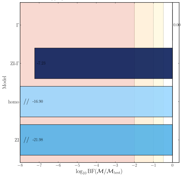
Aggregate across three conditions: contacts
