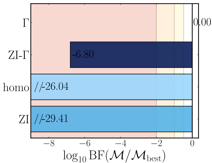
Contacts: aggregate \log_{10} BF across conditions
