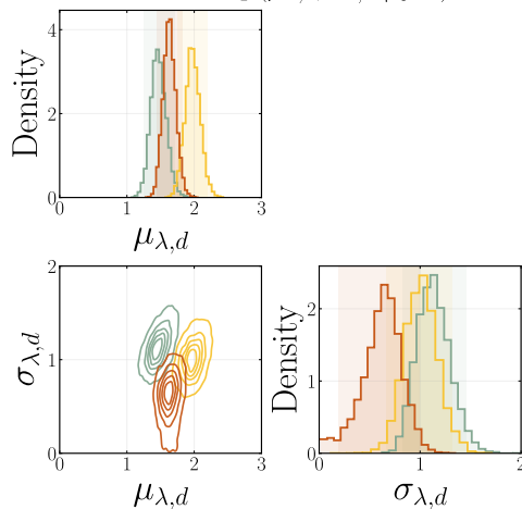
Donor 2 — p(\mu_{\lambda,d}, \sigma_{\lambda,d} \mid y_{\text{kill}})
