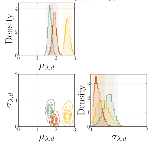
Donor 3 — p(\mu_{\lambda,d}, \sigma_{\lambda,d} \mid y_{\text{kill}})
