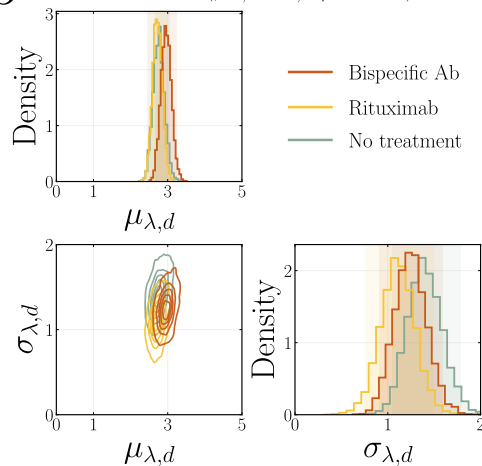
b Donor 2 — p(\mu_{\lambda,d}, \sigma_{\lambda,d} \mid y_{\text{contact}})
