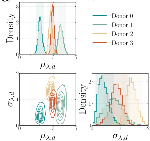
a No treatment — p(\mu_{\lambda,d}, \sigma_{\lambda,d} \mid y_{\text{contact}})
