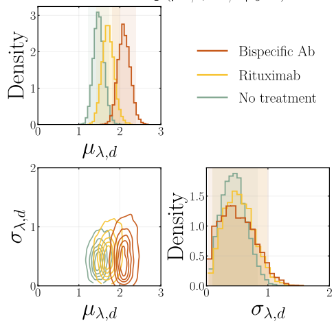
c Donor 1 — p(\mu_{\lambda,d}, \sigma_{\lambda,d} \mid y_{\text{kill}})
