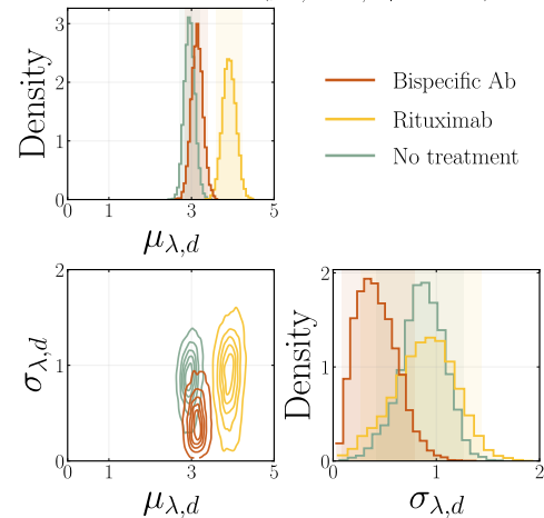
Donor 3 — p(\mu_{\lambda,d}, \sigma_{\lambda,d} \mid y_{\text{contact}})
