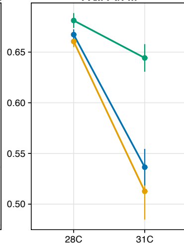
PAM Fv/Fm
