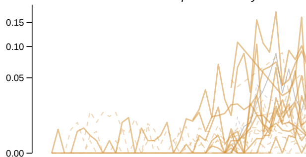
Semicossyphus pulcher – Density
