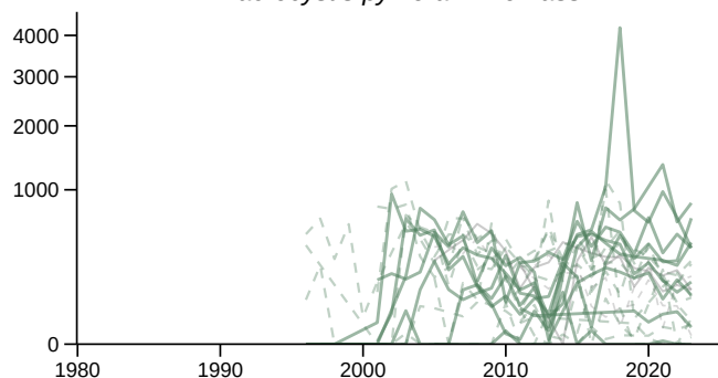
Macrocystis pyrifera – Biomass
