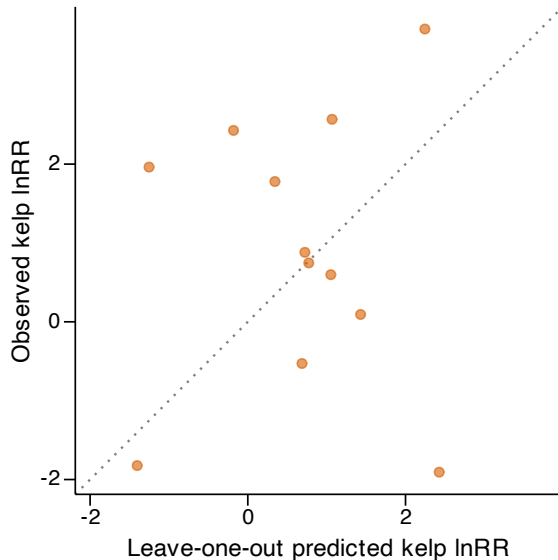
b Can we predict it? LOO-CV R^2 = -0.395
